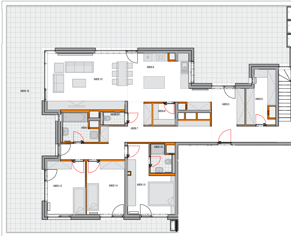
A809_9np M 1: 75
