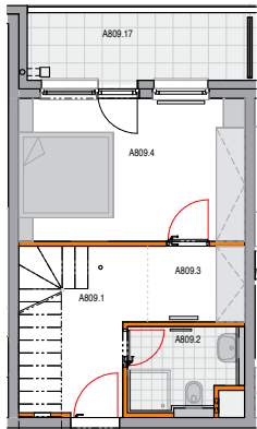
A809_8np M 1: 75
